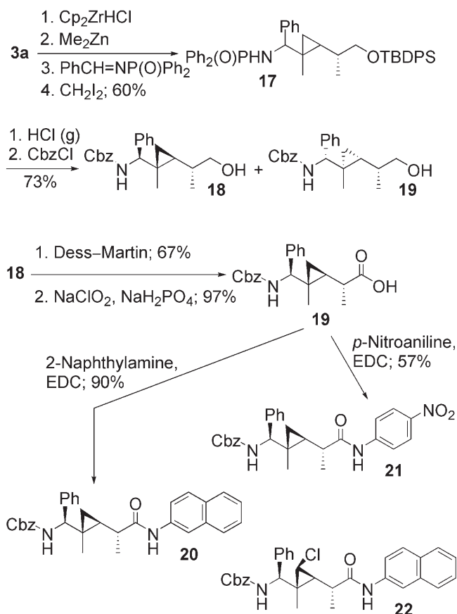
Scheme 6. Synthesis of methyl-substituted CPDIs.
