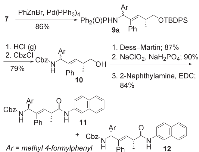
Scheme 4. Negishi cross-coupling for the synthesis of phenyl-substituted TEADIs.
