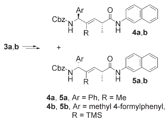
Scheme 2. Synthesis of methyl- and TMS-substituted TEADIs.
