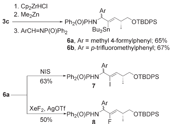
Scheme 3. Introduction of the fluoro- and iodoalkene moieties by electrophilic halogenation of stannylated alkenes.
