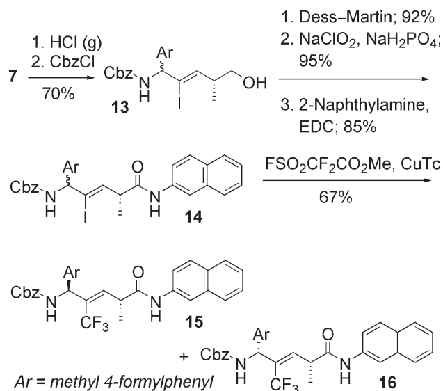
Scheme 5. Synthesis of trifluoromethyl-substituted TEADIs from iodide 14 .
