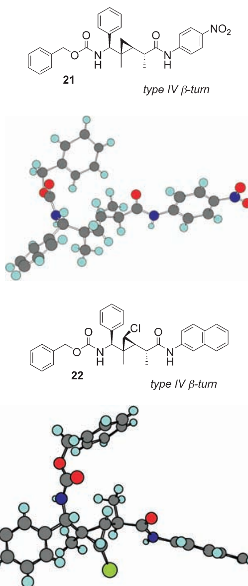
Figure 4. X-ray structures of CPDIs 21 and 22 .
