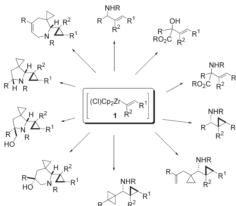
Figure 2. Examples for synthetic scaffolds that are available by addition of alkenylzirconocenes to imines and carbonyl compounds.
