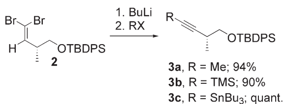
Scheme 1. Synthesis of chiral internal alkynes.
