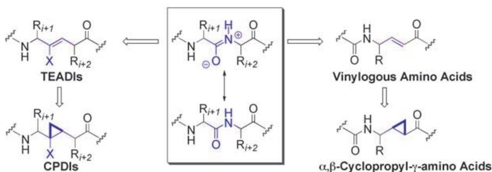
Figure 1. The structural and electronic features of peptide bonds served as inspiration for the design of trisubstituted ( E )-alkene peptide isosteres (TEADIs) and cyclopropane dipeptide isosteres ( \psi [Cp], CPDIs), which are related to backbone-extended vinylogous amino acids and \alpha,\beta -cyclopropyl- \gamma -amino acids.
