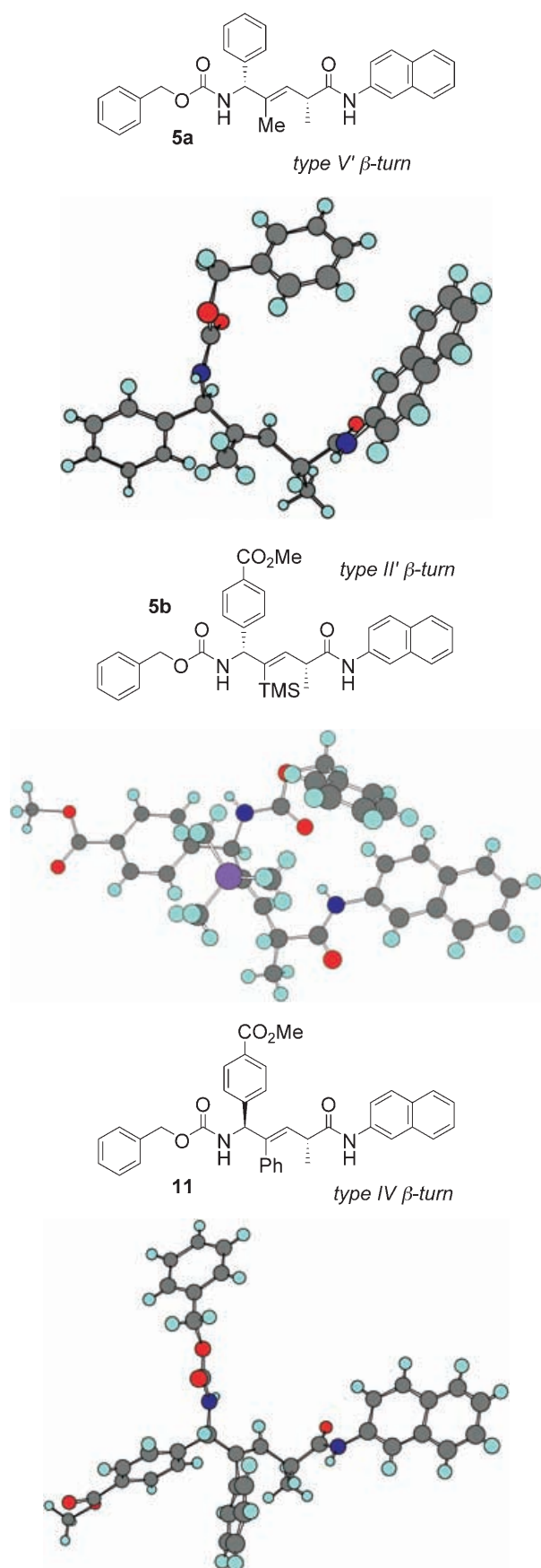
Figure 3. X-ray structures of TEADIs 5a , 5b , and 11 .
